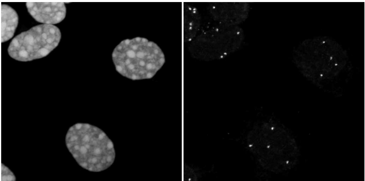
(a) Nucleus
