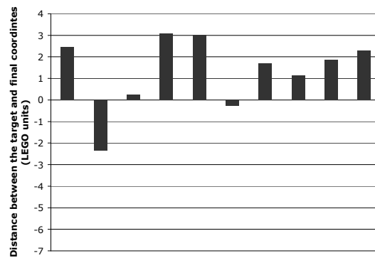
Figure 2 Results of the targeting accuracy tests of the LEGO robot. In each graph, the x-axis shows the results from each of the ten targets. The y-axis shows the distance between the target coordinate and the final needle position in the x, y and z directions for figures A, B and C, respectively.
