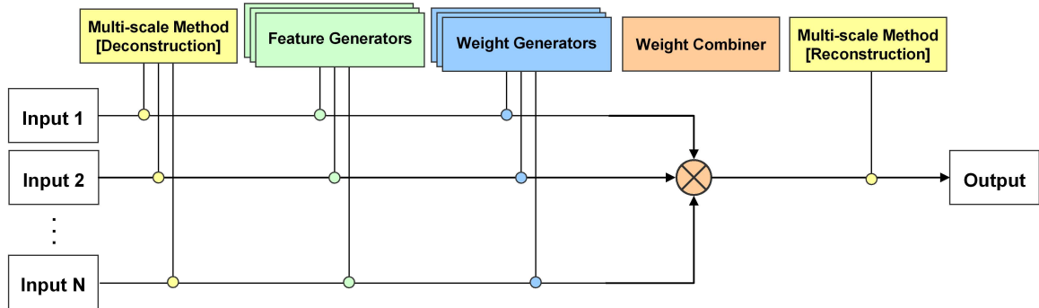
Figure 2: Generalised Image Fusion Toolkit (GIFT) architecture diagram.
